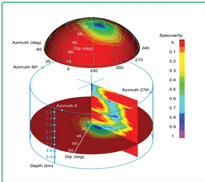
“Specularity” cylindrical directional angle gather
