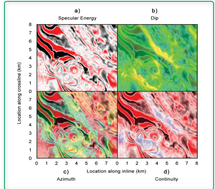
Depth slice throughout 3D image: Specular weighted energy stack, and with an overlay of dip, azimuth, and continuity.
